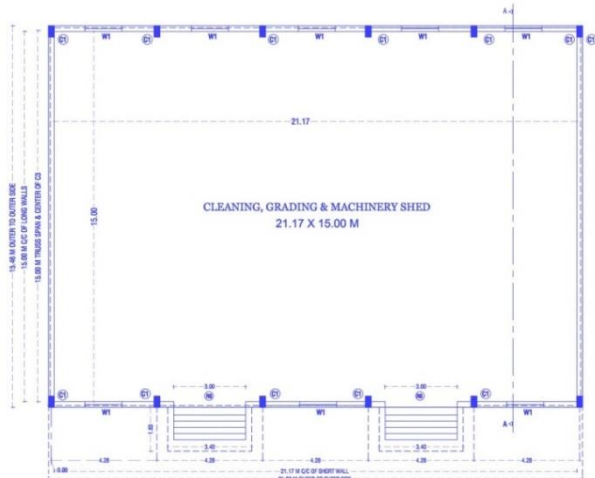
CLEANING ,GRADING & MACHINERY PLANT SHED PLAN
