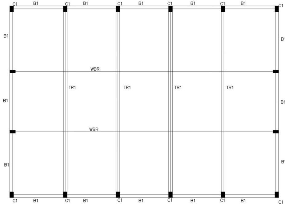
PLAN AT TRUSS TIE LEVEL
