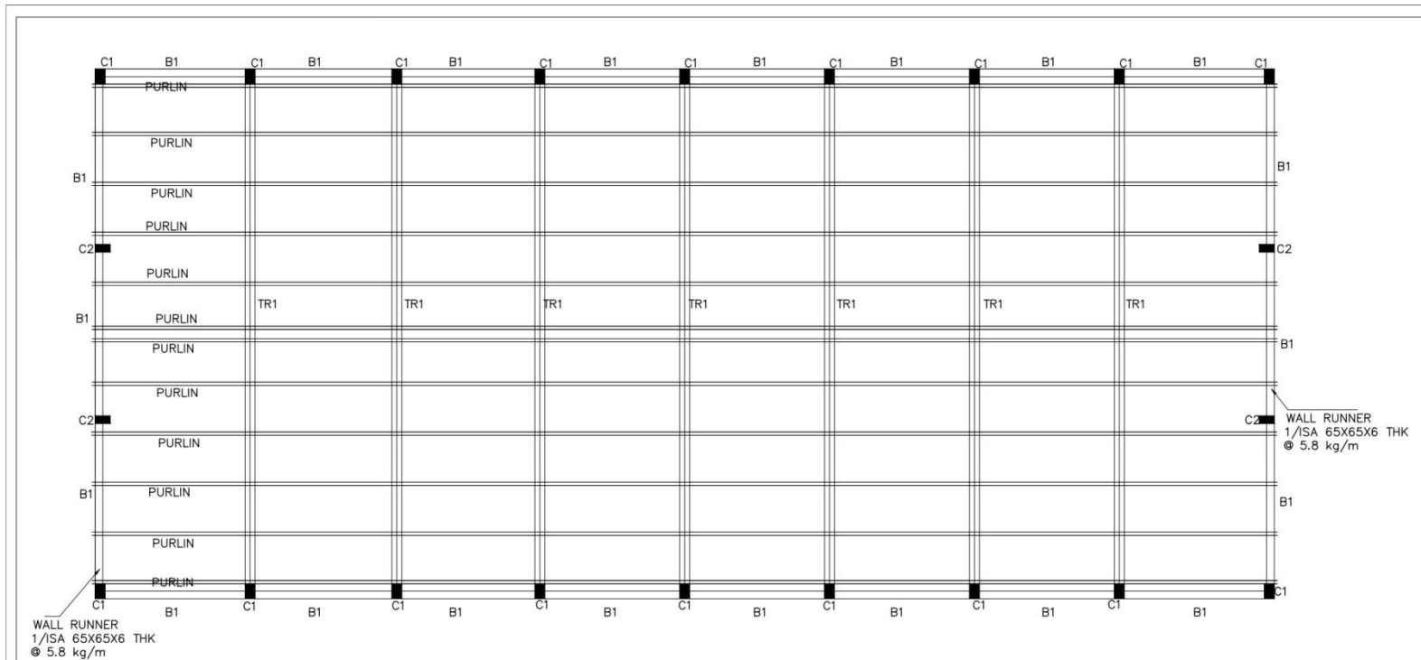
KEY PLAN (LAYOUT OF TRUSS AND PURLIN )
