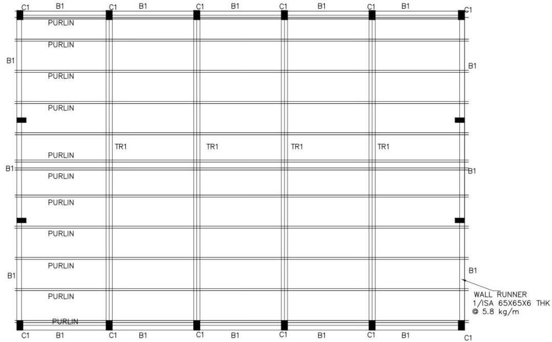
PLAN AT TRUSS TIE LEVEL
